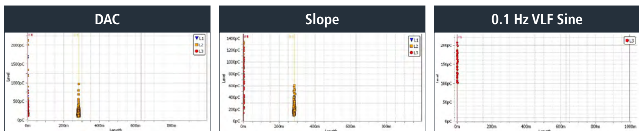
Partial discharge mapping for all excitation voltages (DAC, VLF CR/Slope, and 0.1 Hz VLF Sine wave) at nominal voltage 1.7 \times U_0 . X-axis is the cable length, Y-axis is the discharge height.
