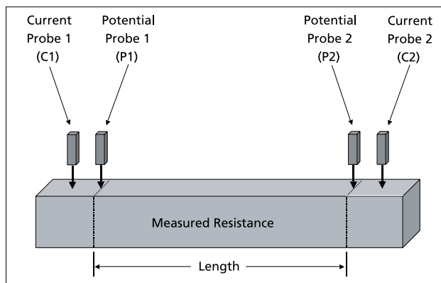
Fig 18: Simplified example of a 4 wire measurement
